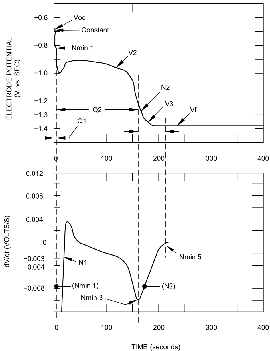
FIGURE G-2. Example SERA differentiated/smoothed curve.
